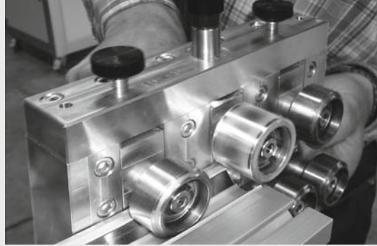
Use the roller assembly tool to bead the aluminium ribs and fix the steel strips in place. Start at the top of the profile then turn the profile and repeat at the bottom.
