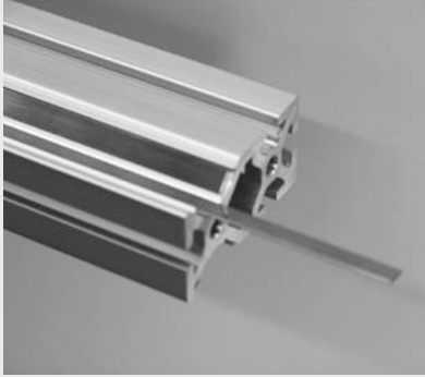
Insert the steel strips into their intended positions.
